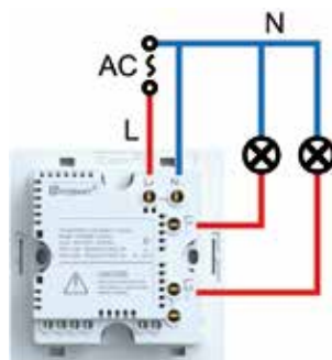
Connection 2: With neutral wire
