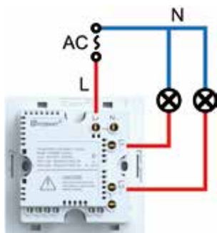
Connection 1: Without neutral wire
